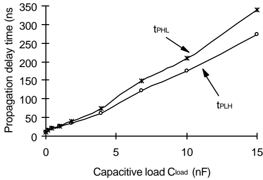
Figure 9 The propagation delay times of the multiplexer.
