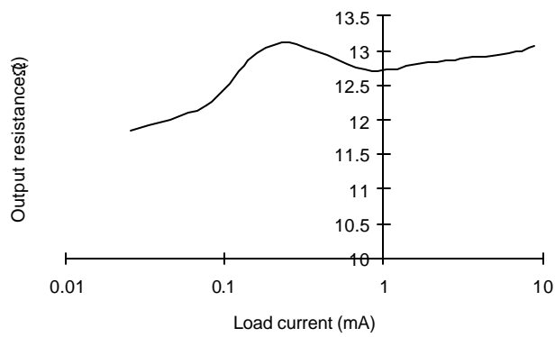
Figure 8 Output resistance vs the load current.
